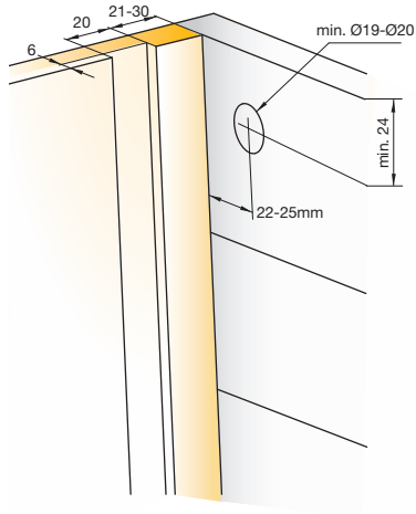
Mounting and drilling details
